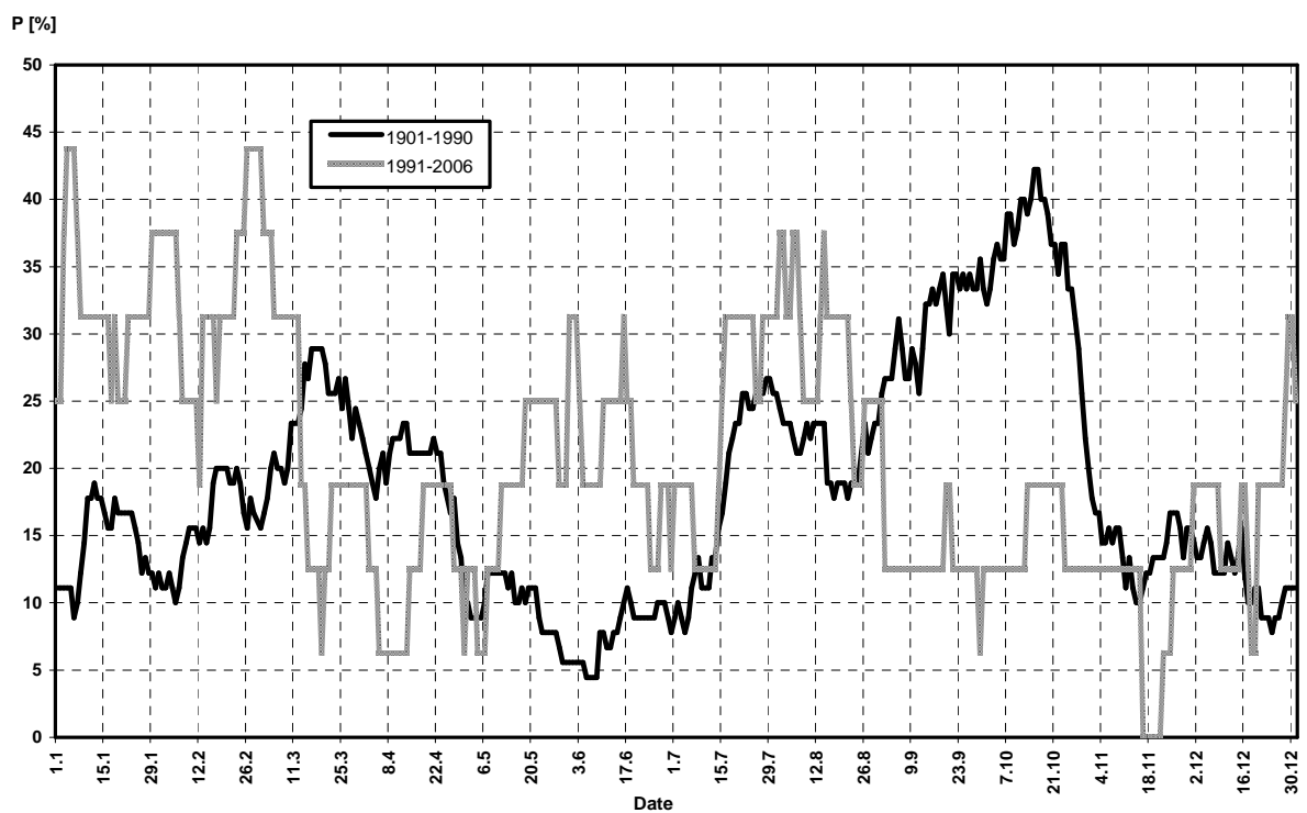
Fig. 5 Annual regime of the probability occurrence of days within PDP (according to criteria 1) in the 1901-1990 and 1991-2006 period in Hurbanovo.
