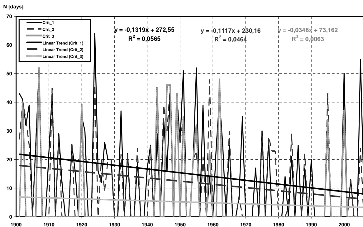
Fig. 13 Number of the precipitation deficit period days (all criteria) during the autumn season (September-November) in Medzilaborce (1901-2006).
