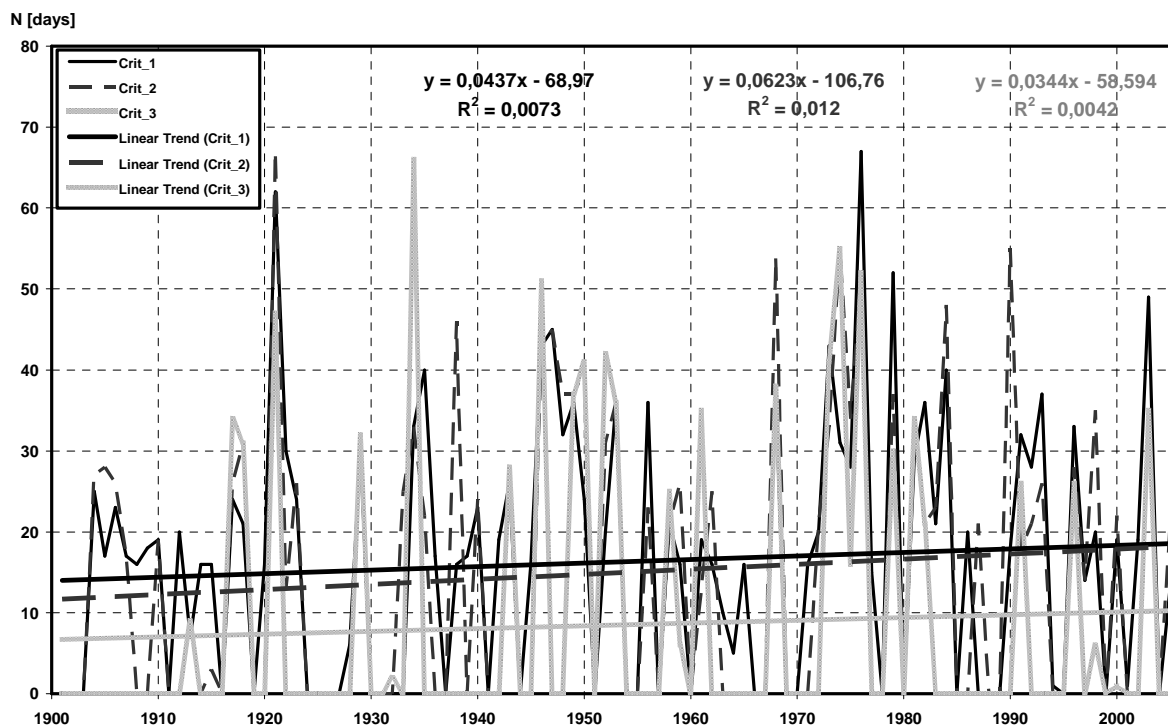
Fig. 7 Number of the precipitation deficit period days (all criteria) during the spring season (March-May) in Hurbanovo (1901-2006).
