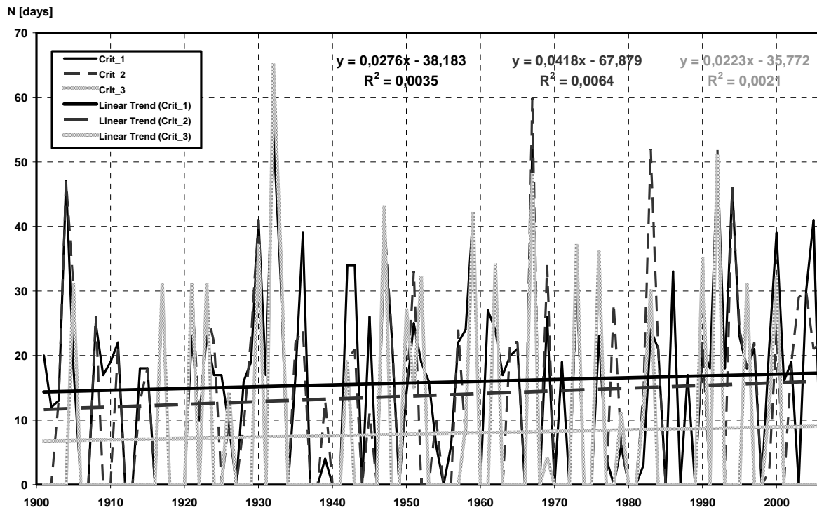
Fig. 8 Number of the precipitation deficit period days (all criteria) during the summer season (June-August) in Hurbanovo (1901-2006).
