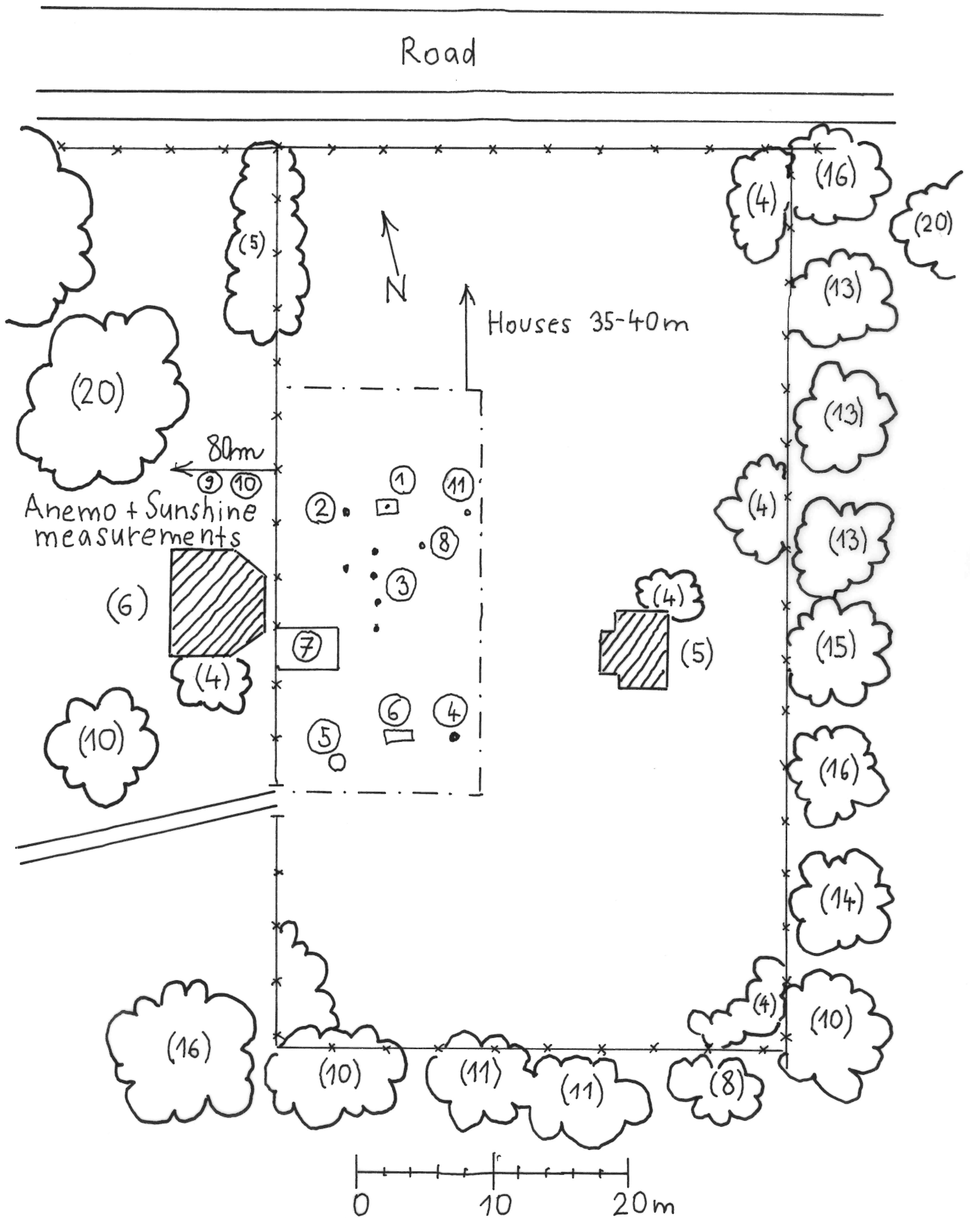
Fig. 4. Station Hurbanovo, ind. 11 858. Layout of the observatory station, updated 30 October 2018
